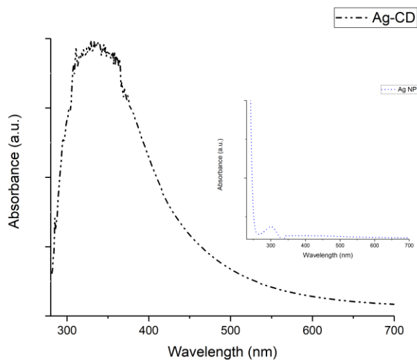
Figure 2. The absorption spectrum of AgNP/CDs. Inset: The absorption spectrum of AgNPs.
