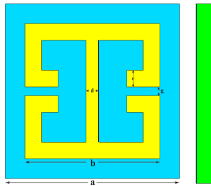
Figure 1. The schematic structure of the proposed terahertz MTM absorber.
