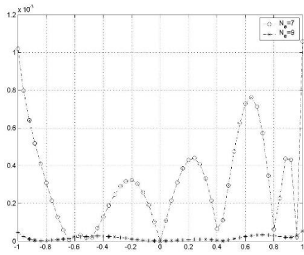
Fig. 5. Comparison of the absolute errors for y_0(t) in Ex. 2.
