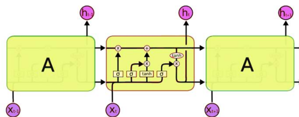
Figure 4: LSTM unit
