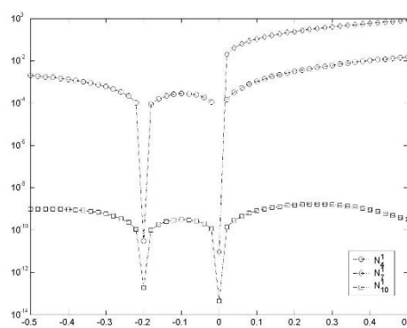
Fig. 14. Comparison of the absolute errors for y_1(t) in Ex. 4.
