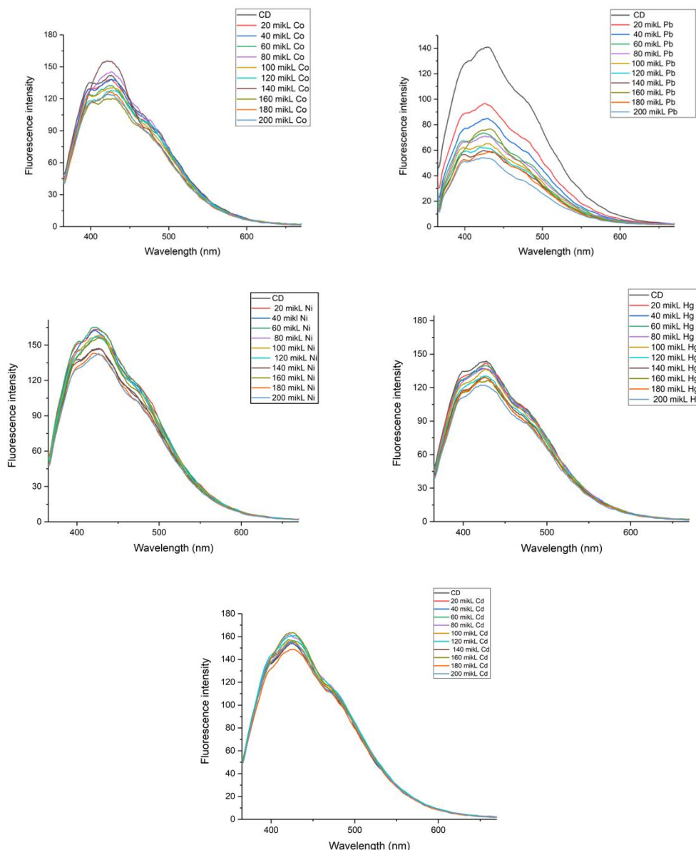
Figure 4. Fluorescence spectra of CDs solutions (1:40 diluted) with different concentrations of Co II, Pb II, Ni II, Hg II, Cd II ions.
