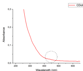
Figure 2. UV-Absorption Spectrum of QDs.
