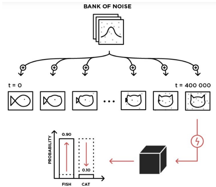
Figure 33: A scheme regarding applying the Boundary Attack [58].
