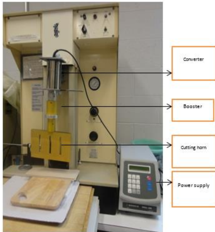
Figure 1. Ultrasonic knife used for experimental design (Sonics& Materials, Inc.)
