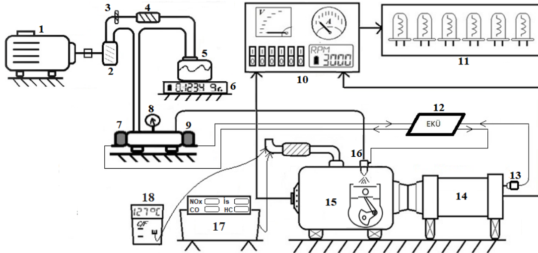
1- Electric motor, 2- High pressure pump, 3- Fuel filter, 4- Feed pump, 5- Fuel tank, 6- Digital scale, 7- Pressure control valve, 8- Manometer, 9- Pressure sensor, 10-Control panel, 11-Load unit, 12- ECU, 13- Encoder, 14- Alternator, 15- Diesel engine, 16- Solenoid injector, 17- Exhaust emission device and opacimeter, 18-Digital multimeter and thermocouple.
