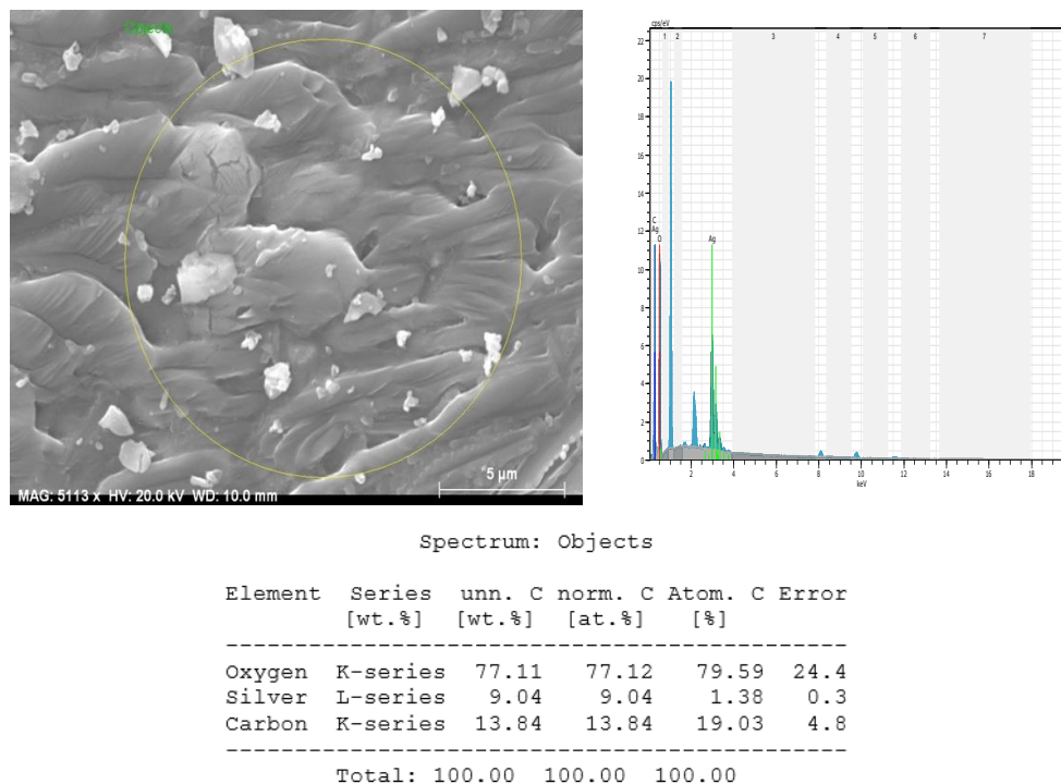
Figure 4. SEM microgram of AgNP/CDs nano hybrids at lower magnification (left image), mapped region for EDX (right image) and EDX results (table).
