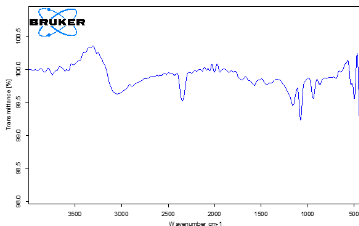
Figure 1. FTIR Spectra of CDs.
