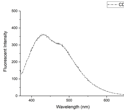
Figure 3. Fluorescence Spectrum of CDs.
