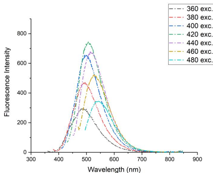
Figure 3. Full-excitation wavelength PL spectra of AgNP/CDs.
